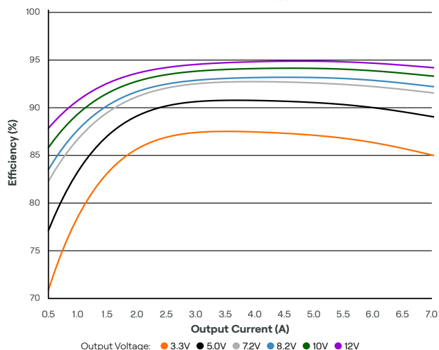
LV Channel Efficiency, V_{bus} 29.6V (8S)
