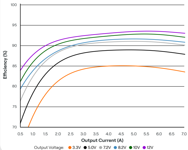
LV Channel Efficiency, V_{bus} 51.8V (14S)
