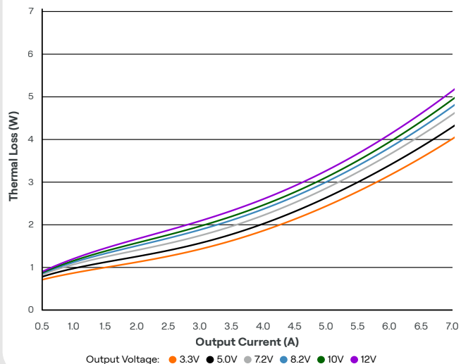
LV Channel Loss, V_{bus} 29.6V (8S)
