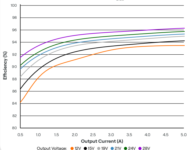
HV Channel Efficiency, V_{bus} 51.8V (14S)
