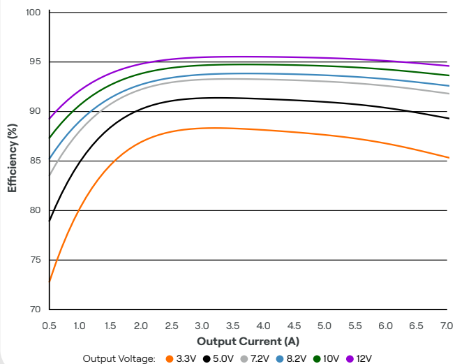
LV Channel Efficiency, V_{bus} 22.2V (6S)
