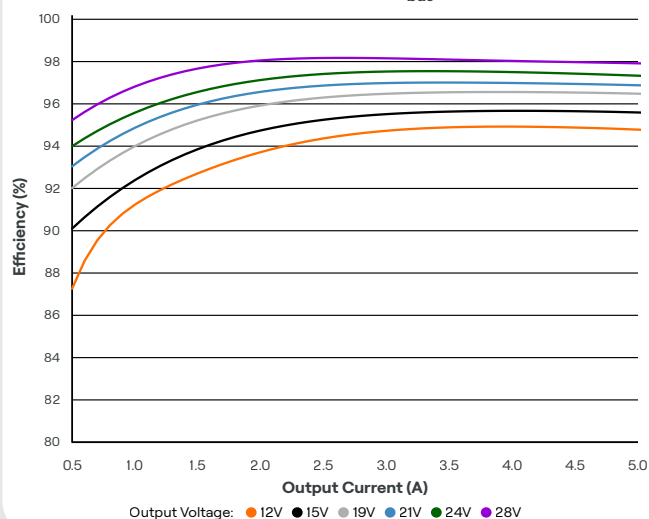
HV Channel Efficiency, V_{bus} 29.6V (8S)
